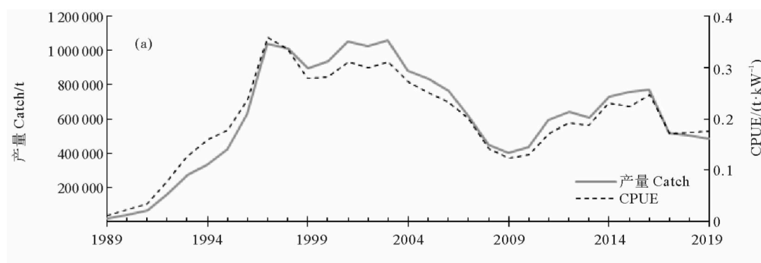
Figure 3. Statistics of catch and CPUE for the anchovy stocks in the Yellow Sea 10
