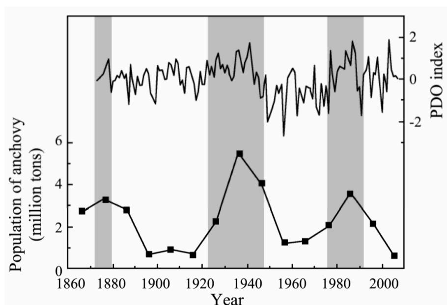
Figure 2. Long-term, reconstructed abundance trends of Japanese anchovy in the Yellow Sea, showing hypothesized relationship to the Pacific Decadal Oscillation Index. 9
